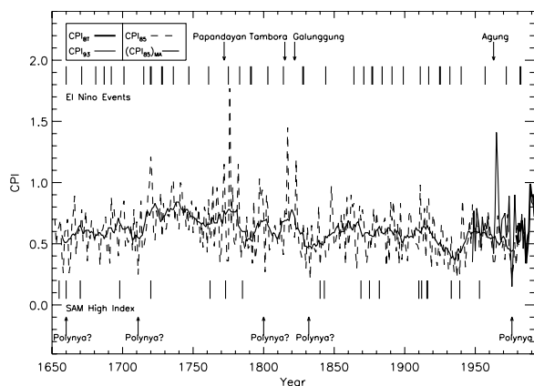
Figure 2. The Cross-Peninsula Index (CPI) calculated from: the frequency of BT patterns ( CPI_{BT} ; heaviest solid line); a regression of the 1993 ice core chemical species onto the CPI_{BT} ( CPI_{93} ; thinnest solid line); and the regression equation applied to the chemical species from the 1985 ice core ( CPI_{85} ; dashed line). The medium solid line shows the 10-point moving average of the CPI_{85} . The bars above and below the plot represent the timings of moderate (thin bar), strong (medium bar) or very strong (thick bar) (top) El Niño events and (bottom) SAM years.
